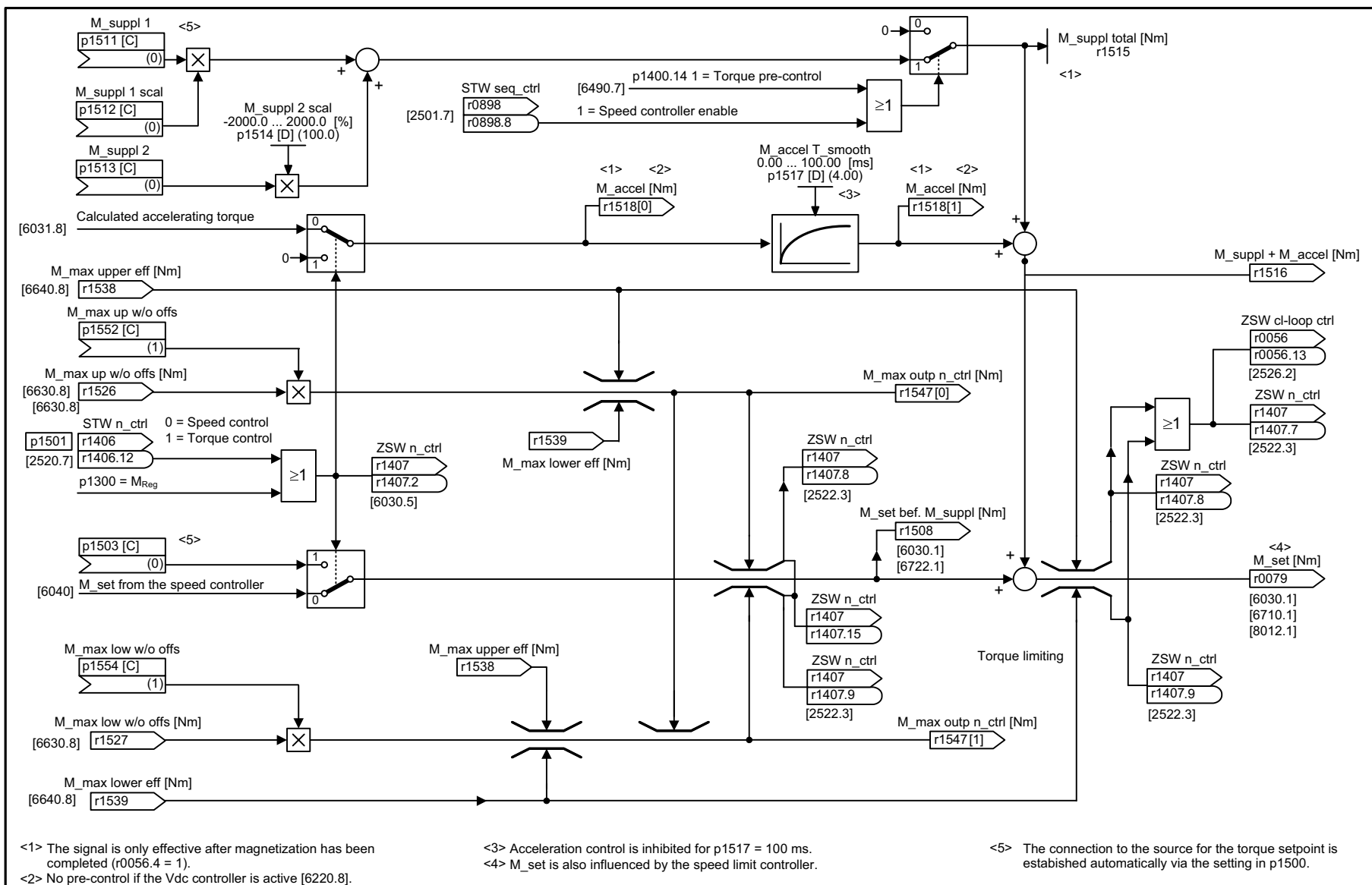
Fig. 2-77 6060 – Torque setpoint
