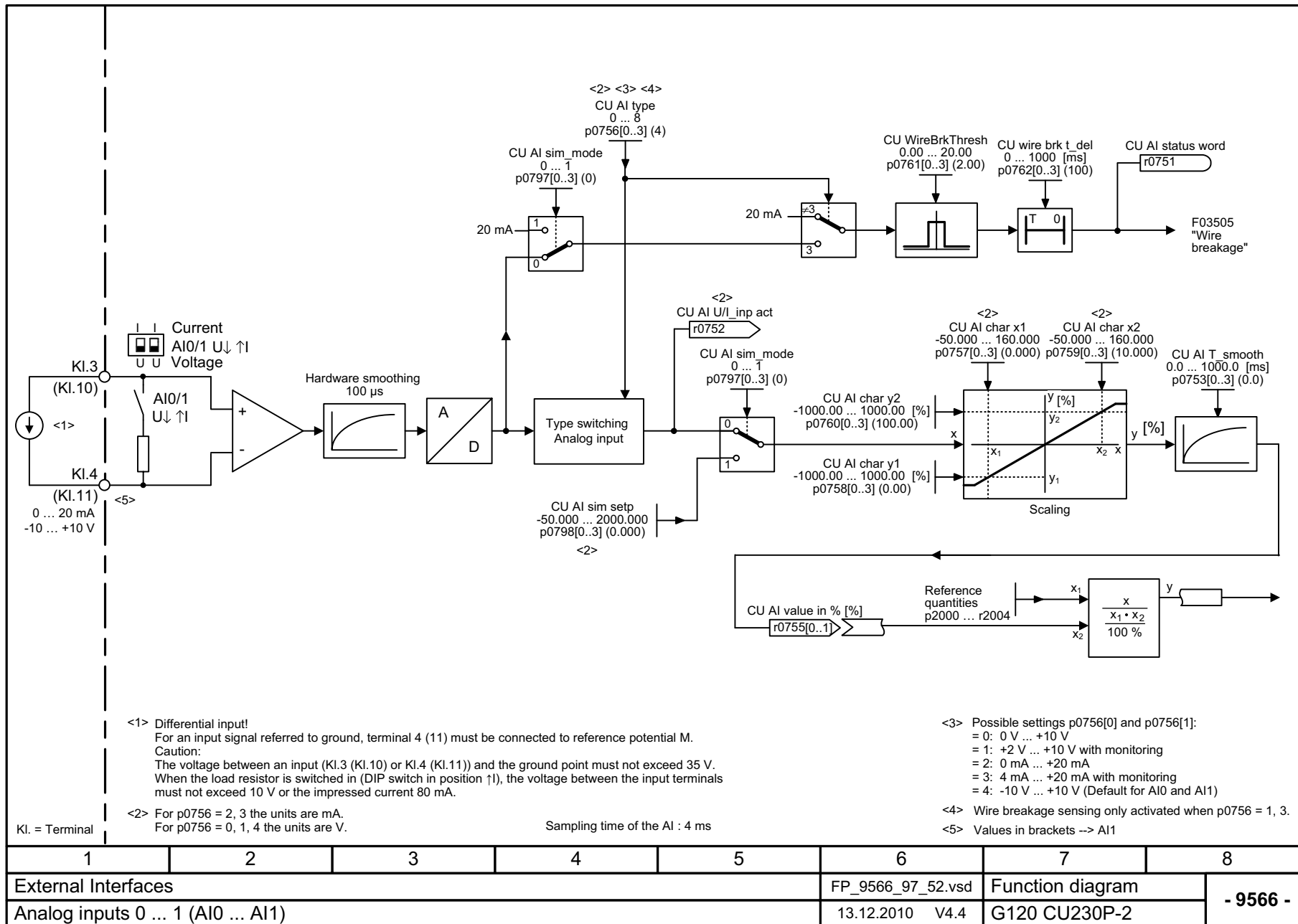
Fig. 2-15 9566 – Analog inputs 0 ... 1 (AI0 ... AI1)
