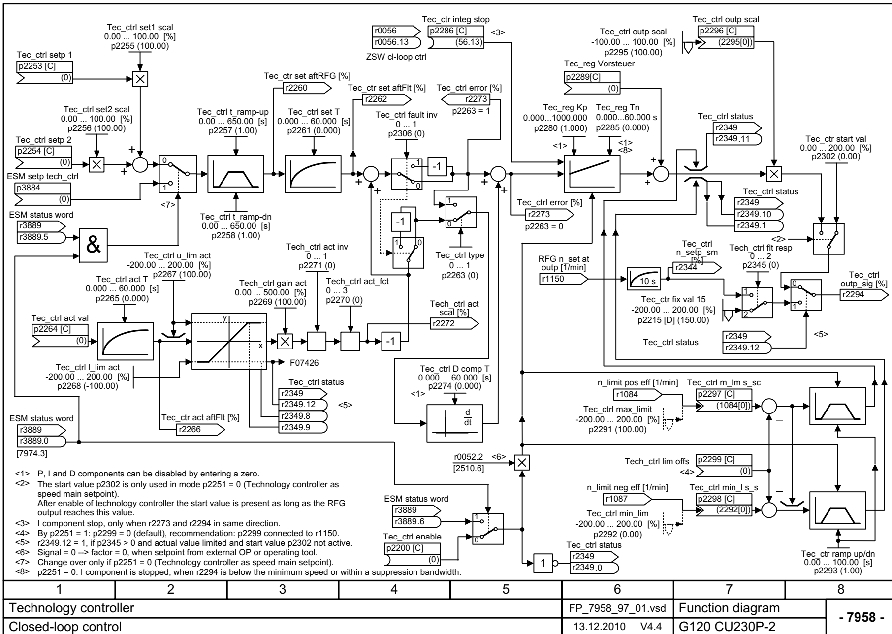
Fig. 2-122 7958 – Closed-loop control
