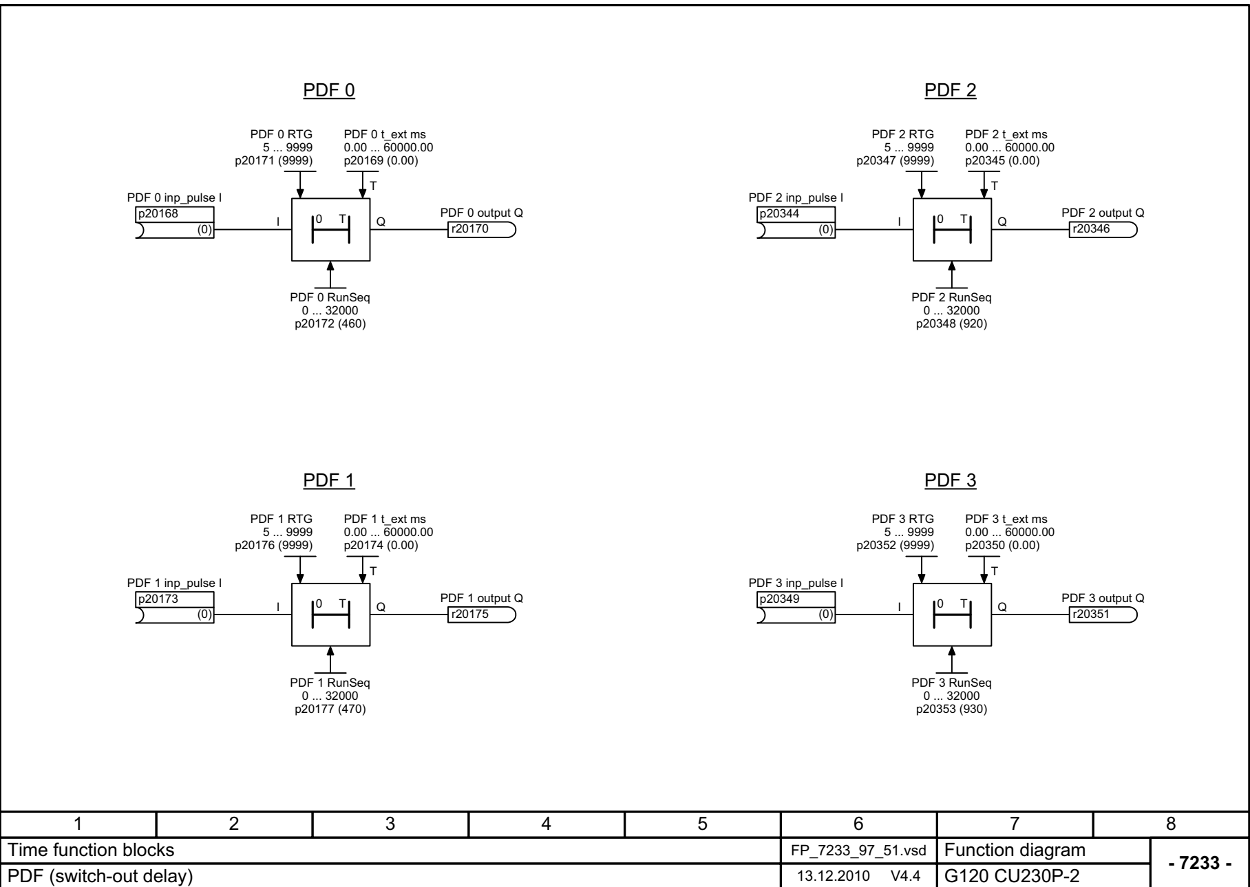
Fig. 2-104 7233 – PDF (switch-out delay)
