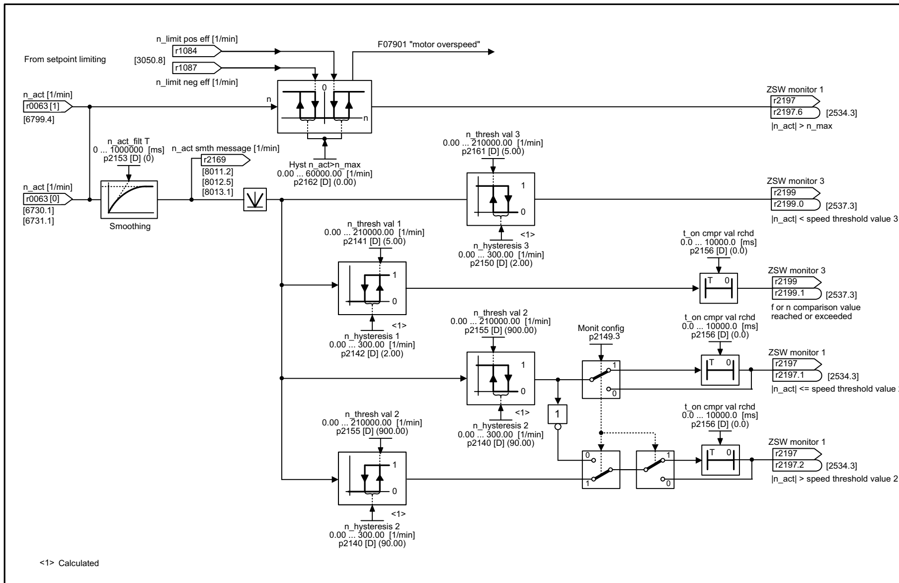
Fig. 2-123 8010 – Speed signals 1
