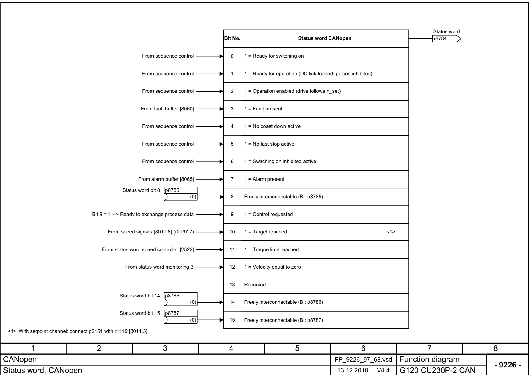
Fig. 2-43 9226 – Status word, CANopen
