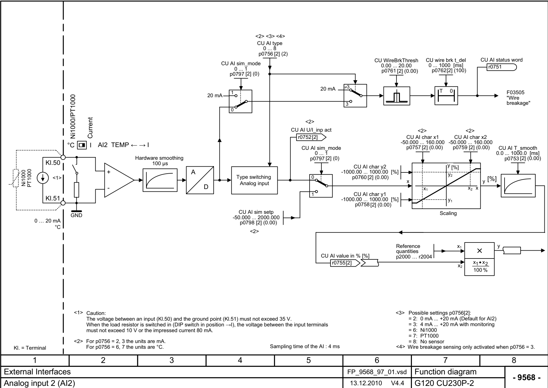
Fig. 2-16 9568 – Analog input 2 (AI2)
