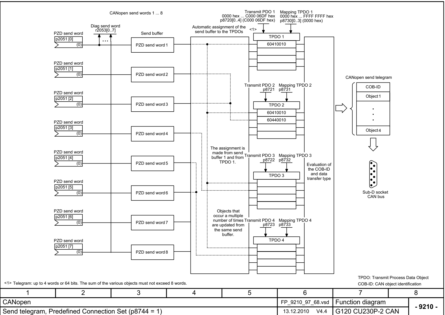
Fig. 2-41 9210 – Send telegram, Predefined Connection Set (p8744 = 1)
