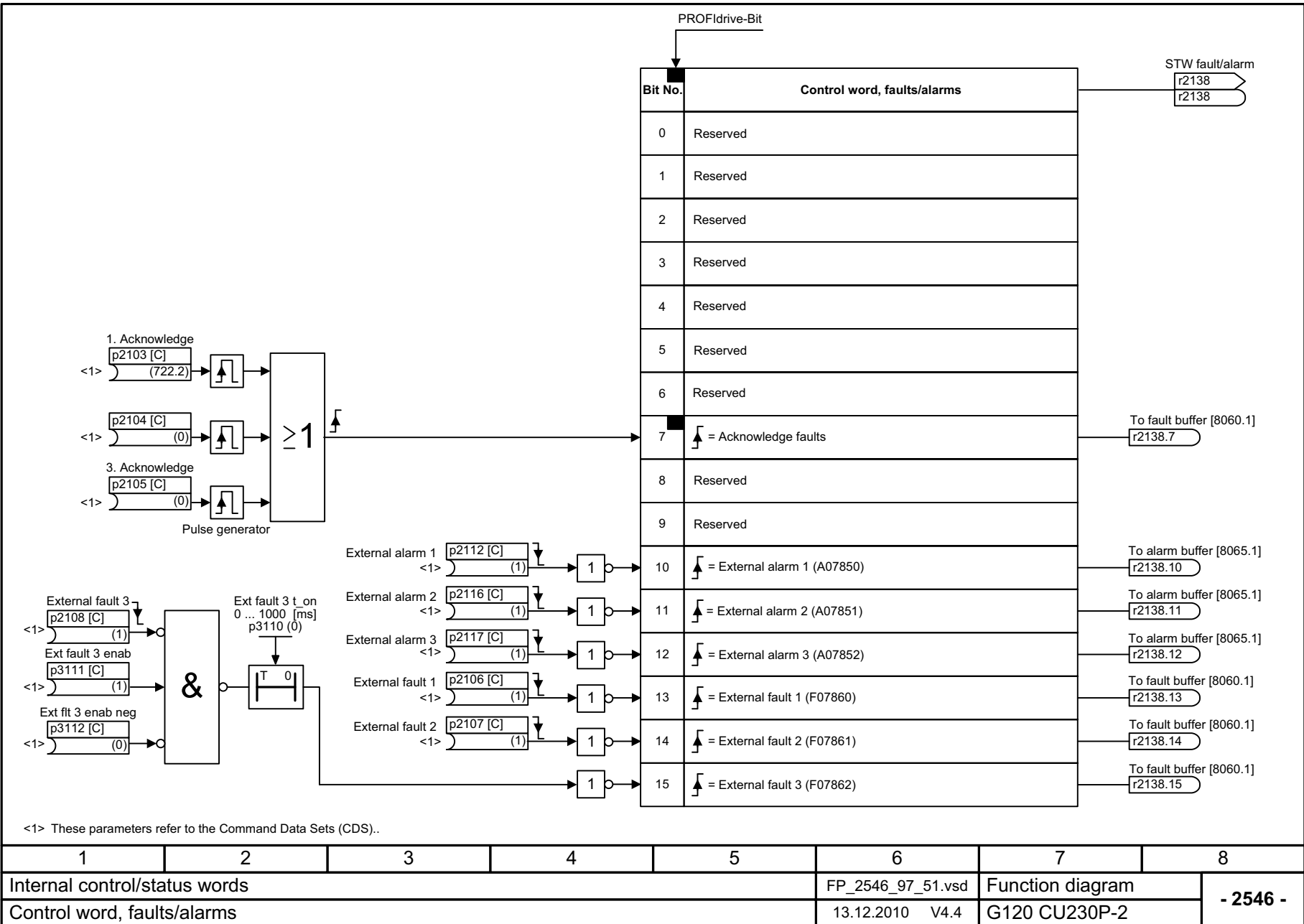
Fig. 2-58 2546 – Control word, faults/alarms
