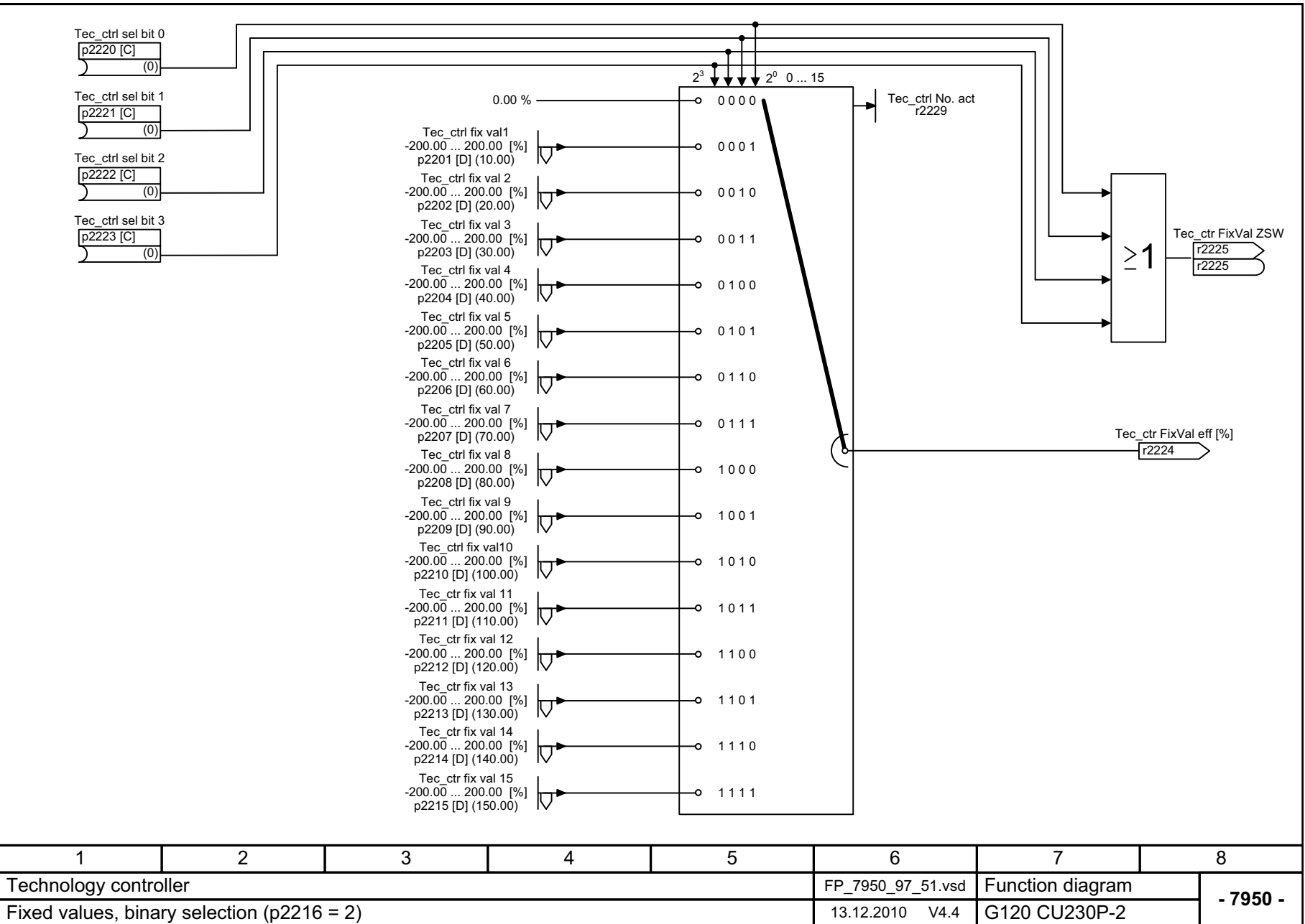
Fig. 2-119 7950 – Fixed values, binary selection (p2216 = 2)
