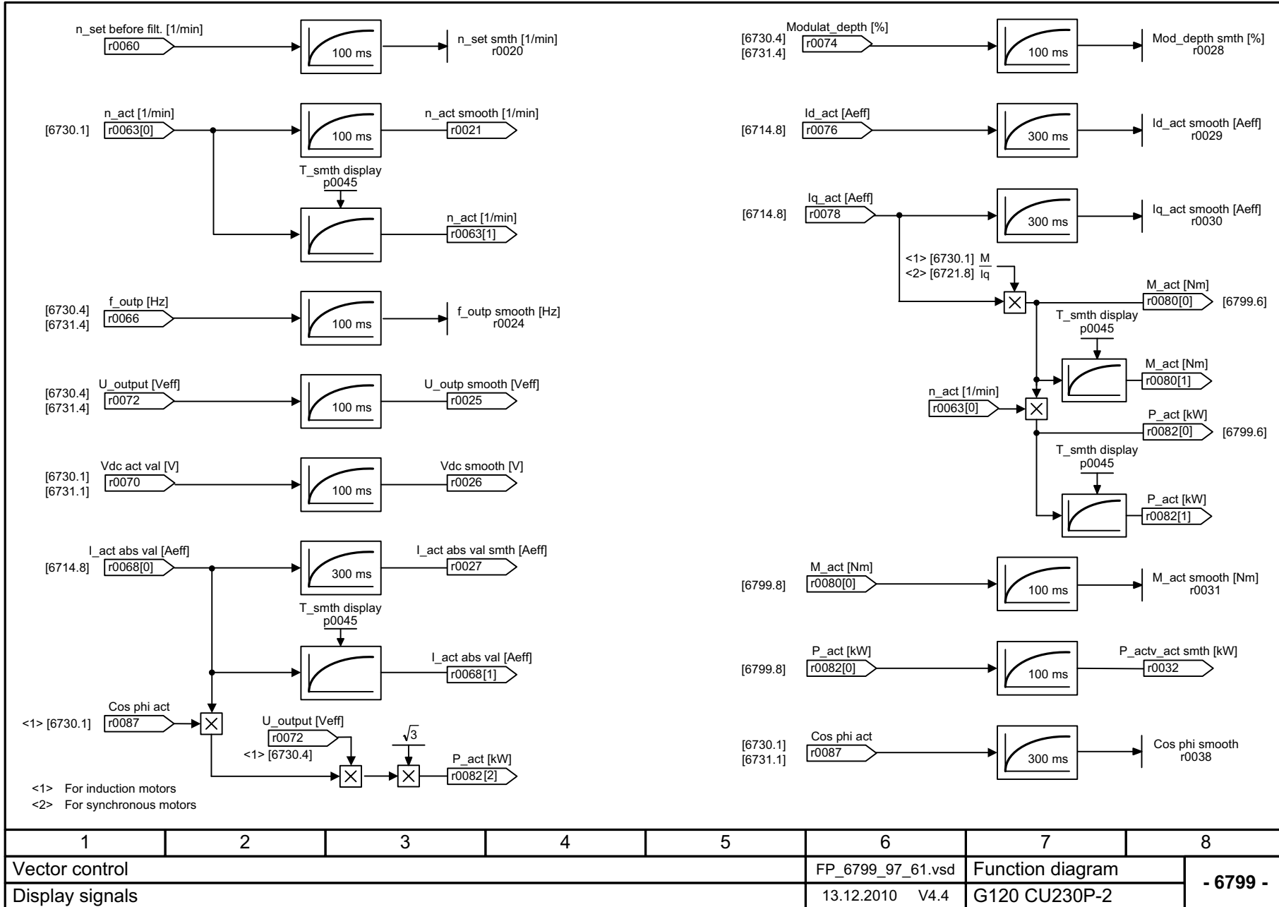
Fig. 2-91 6799 – Display signals
