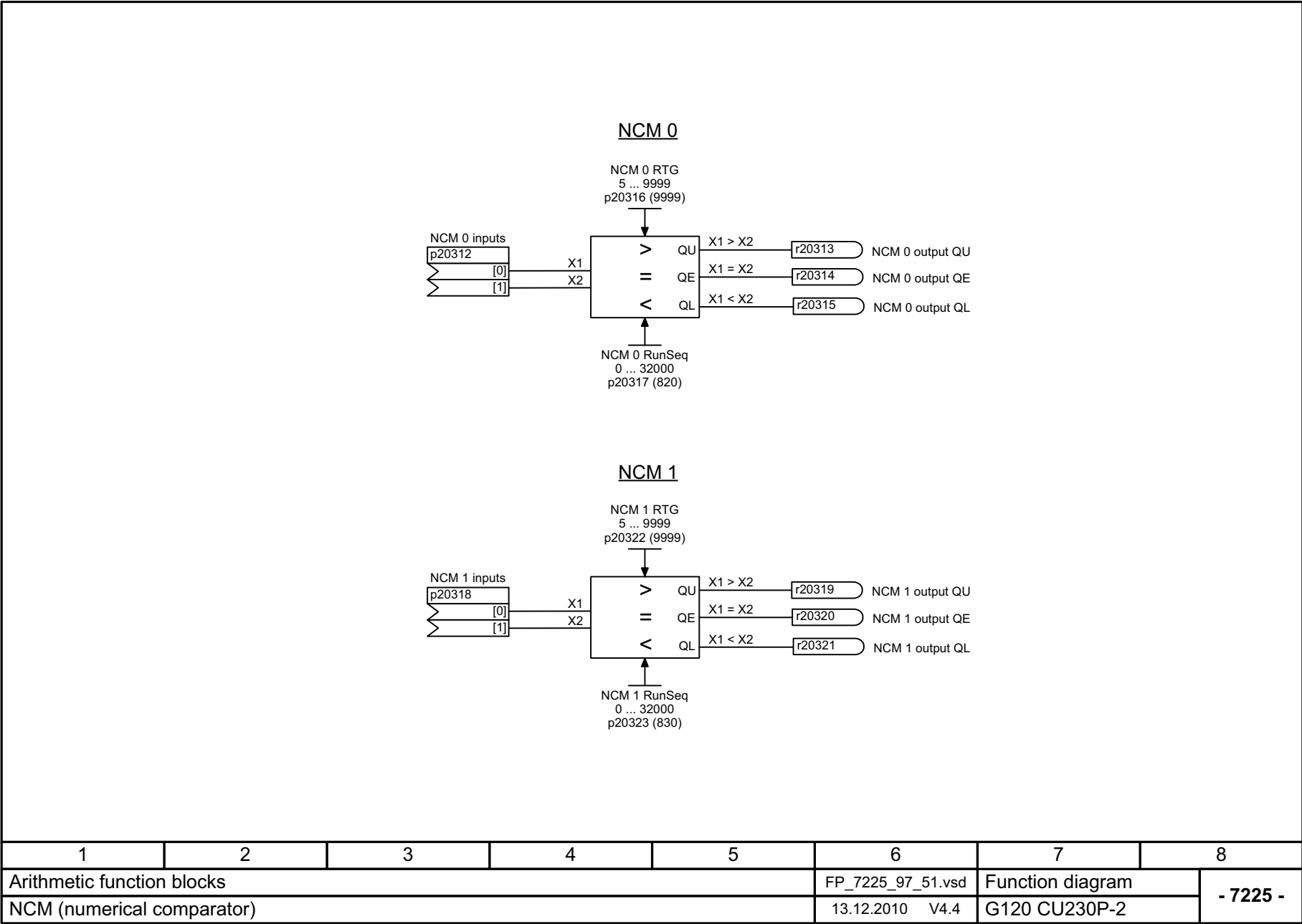
Fig. 2-100 7225 – NCM (numerical comparator)
