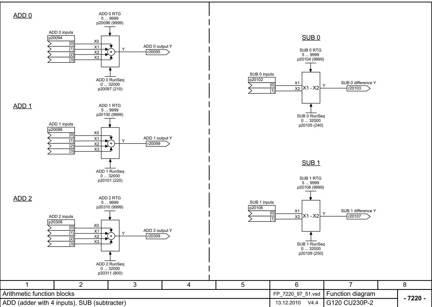
Fig. 2-97 7220 – ADD (adder with 4 inputs), SUB (subtractor)
