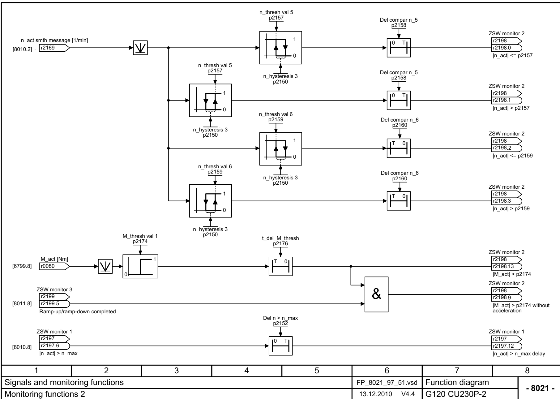
Fig. 2-131 8021 – Monitoring functions 2
