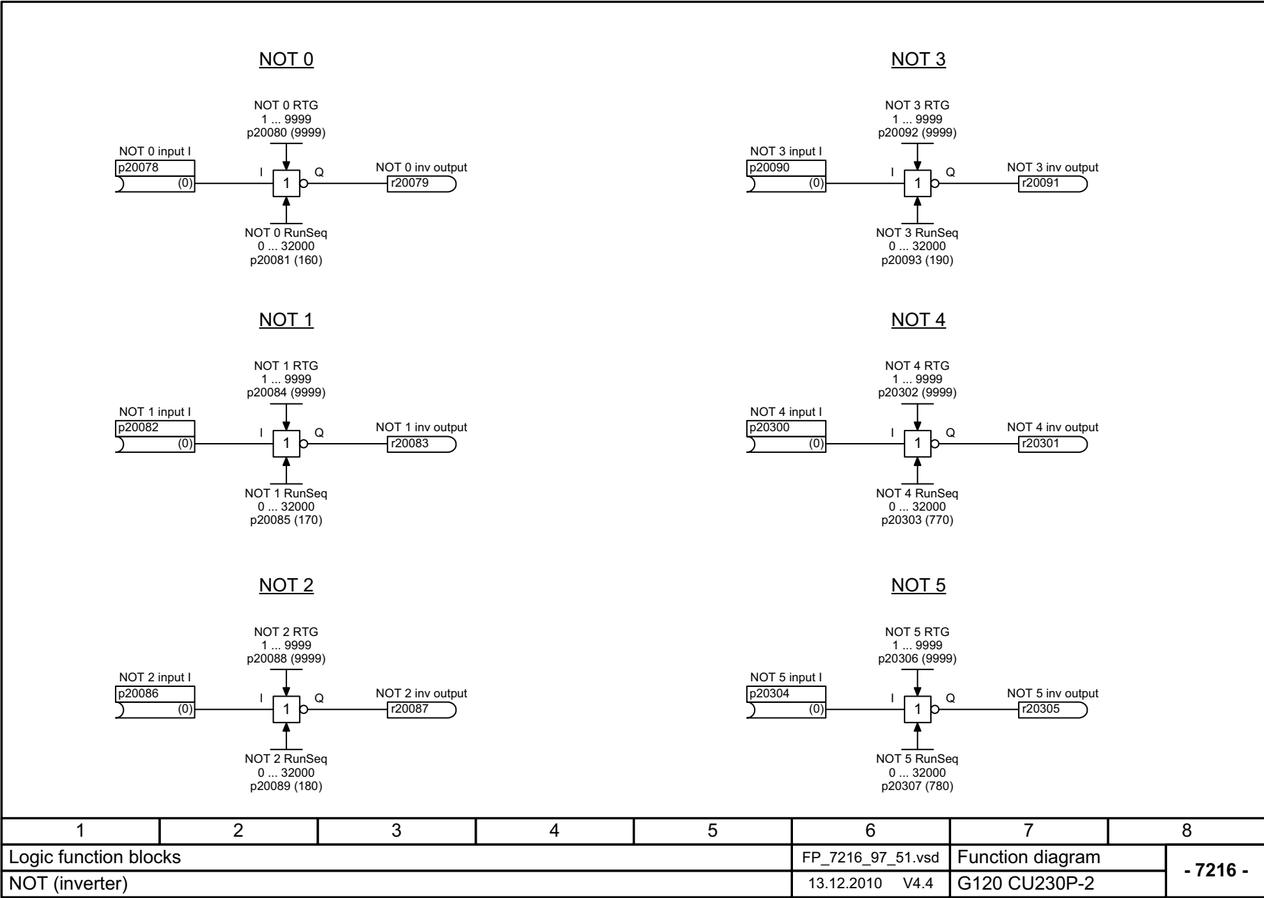
Fig. 2-96 7216 – NOT (inverter)
