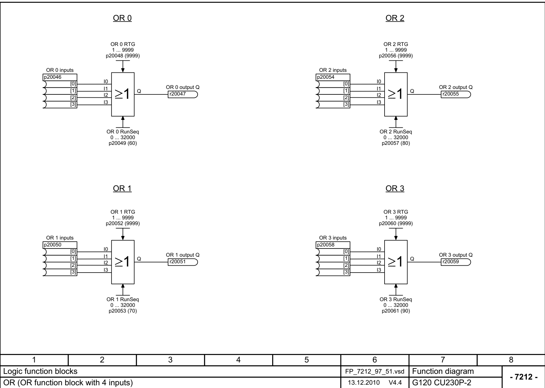
Fig. 2-94 7212 – OR (OR function block with 4 inputs)
