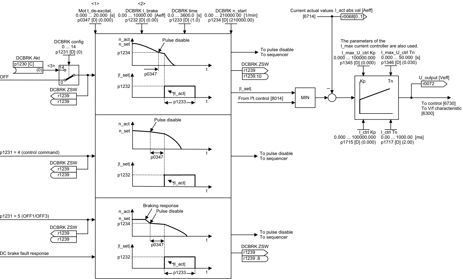
Fig. 2-112 7017 – DC brake (p0300 = 1)
