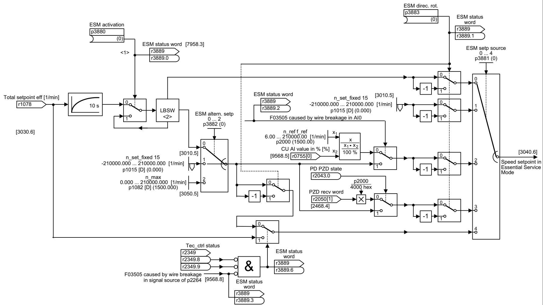
Fig. 2-115 7973 – Essential Service Mode
