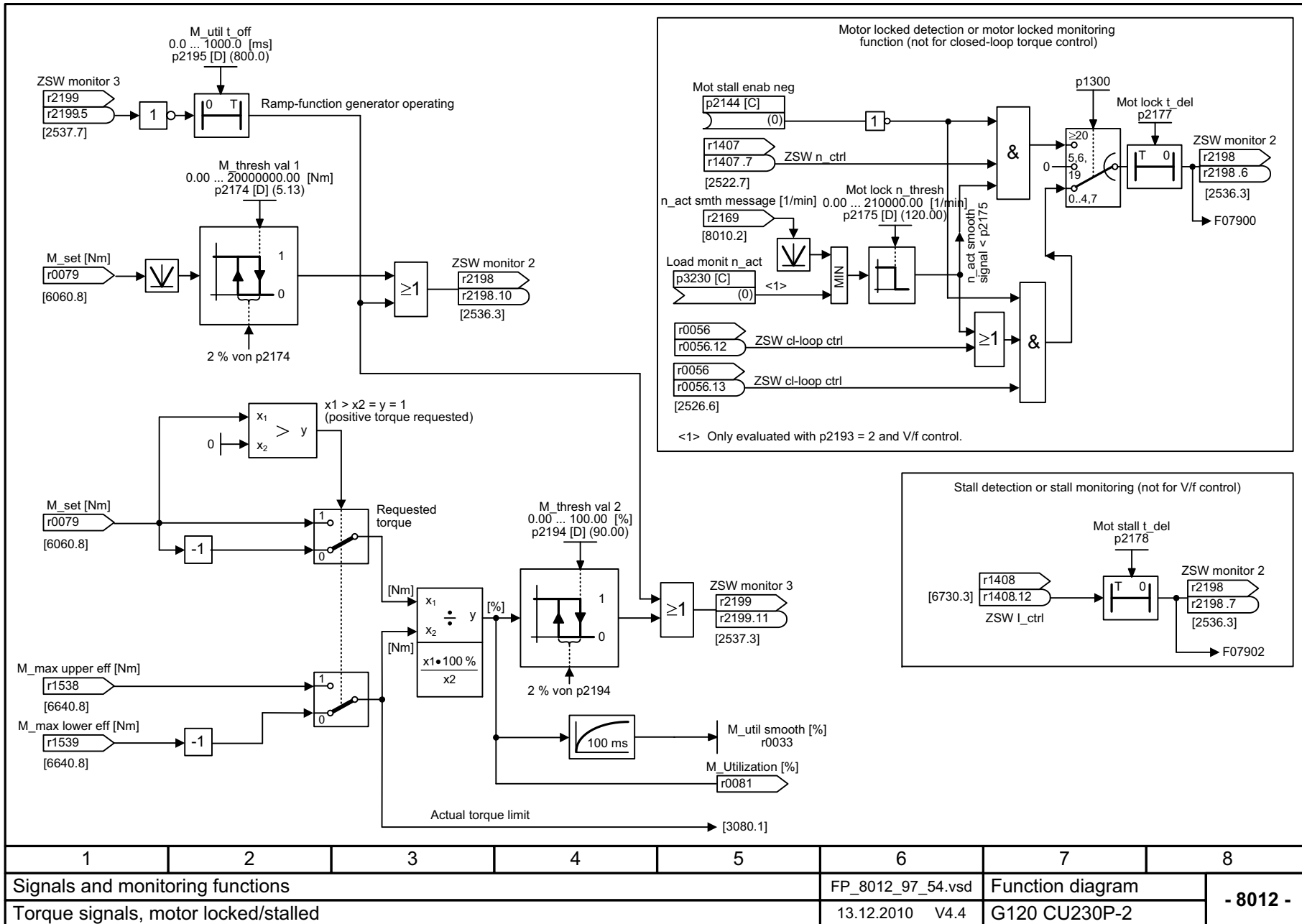
Fig. 2-125 8012 – Torque signals, motor locked/stalled
