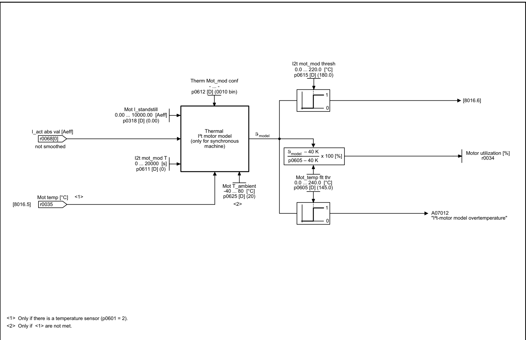
Fig. 2-129 8017 – Thermal I²t motor model (PEM, p0300 = 2xx)
