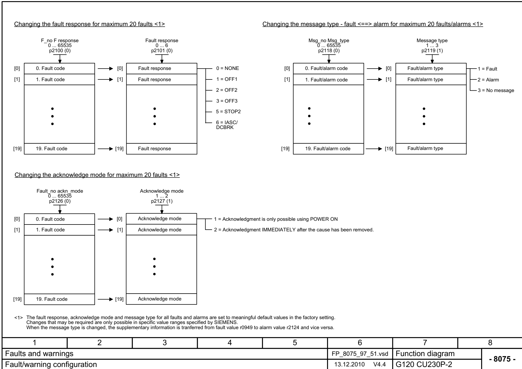
Fig. 2-135 8075 – Fault/warning configuration
