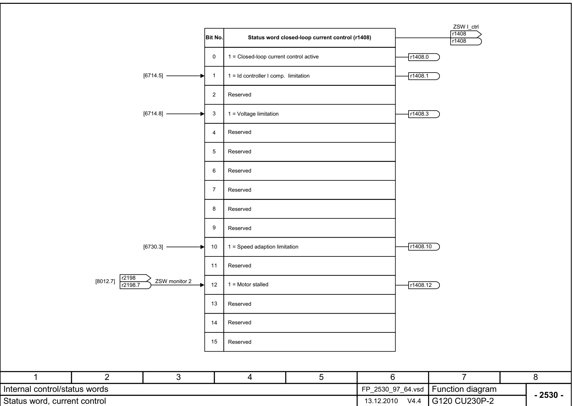
Fig. 2-54 2530 – Status word, current control
